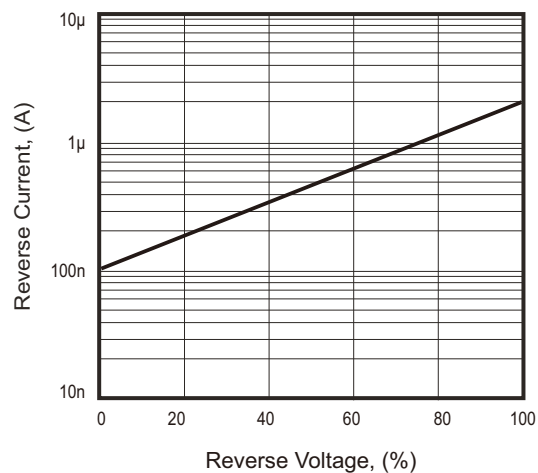
Fig.2 - Reverse Characteristics
